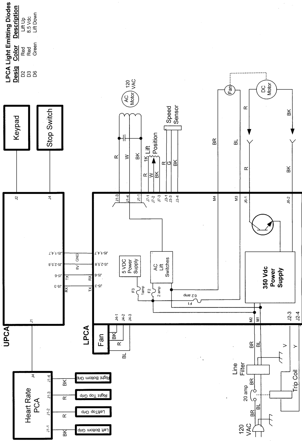
C966-120 PWM Treadmill
